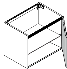
Wall mounted vanity unit with 1 door Base portlavabo sospesa con 1 anta W 60 cm D 38/46/51,5 cm
